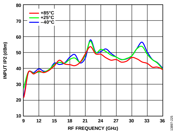
Figure 25. Input IP2 vs. RF Frequency over Various Temperatures, P_{LO} = 15 dBm
