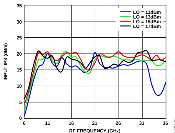
Figure 51. Input IP3 vs. RF Frequency over Various LO Drives
