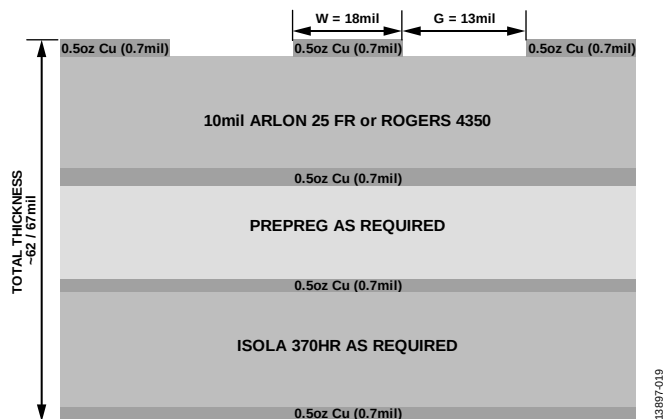
Figure 94. Evaluation Board Cross Sectional View
