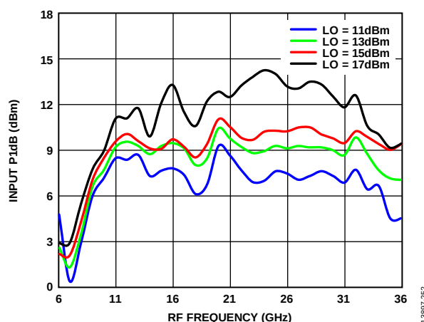
Figure 52. Input P1dB vs. RF Frequency over Various LO Drives
