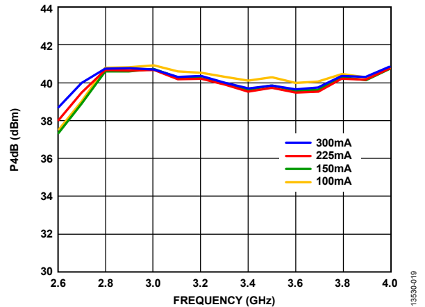
Figure 19. Output Power for 4 dB Compression ( P_{4dB} ) vs. Frequency at Various Supply Currents
