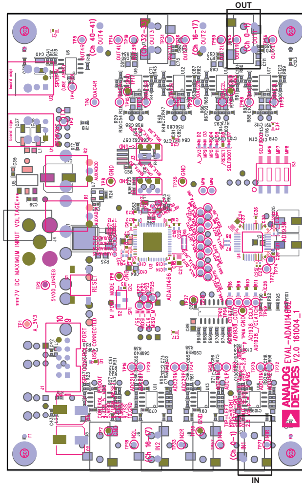
Figure 13. Location of Stereo Output OUT1 (J10) and Stereo Input IN1 (J9), Rotated 90°
