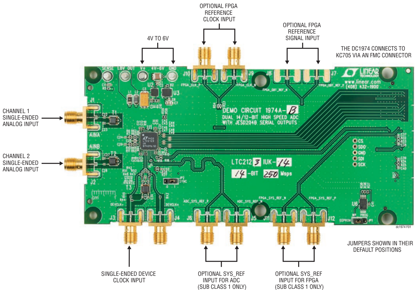
Figure 1. DC1974 Setup
