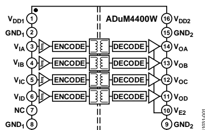
Figure 1. ADuM4400W
