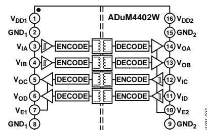
Figure 3. ADuM4402W
