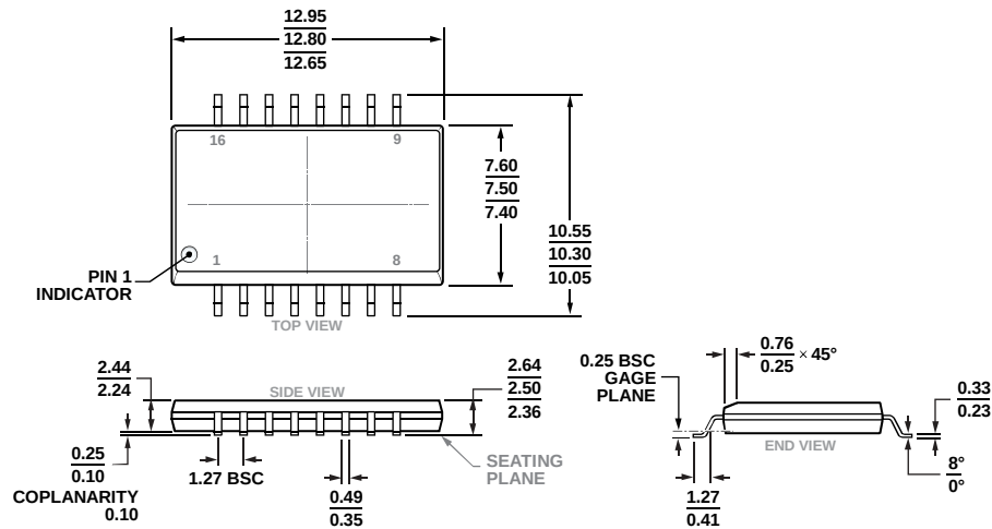
Figure 23. 16-Lead Standard Small Outline Package [SOIC_IC] Wide Body (RI-16-2)
