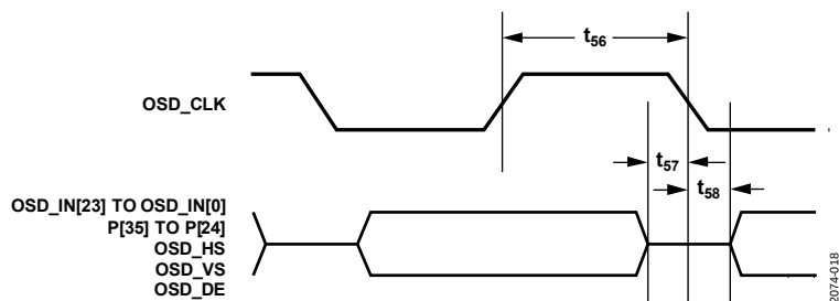
Figure 17. SDR Video Data and Control Output Timing (Data Launched on Falling Edge)
