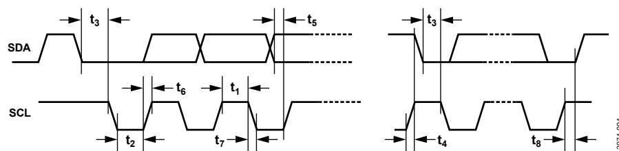
Figure 3. I²C Timing
