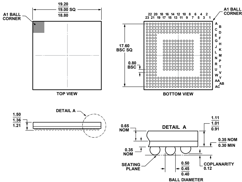
Figure 38. 425-Ball Chip Scale Package Ball Grid Array [CSP_BGA] (BC-425-1) Dimensions shown in millimeters
