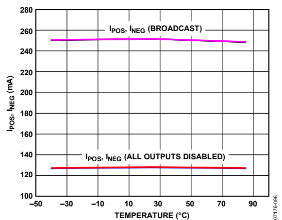
Figure 45. ADV3200 Supply Current vs. Temperature
