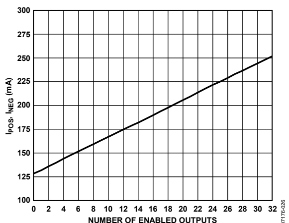
Figure 46. ADV3200 Supply Current vs. Enabled Outputs
