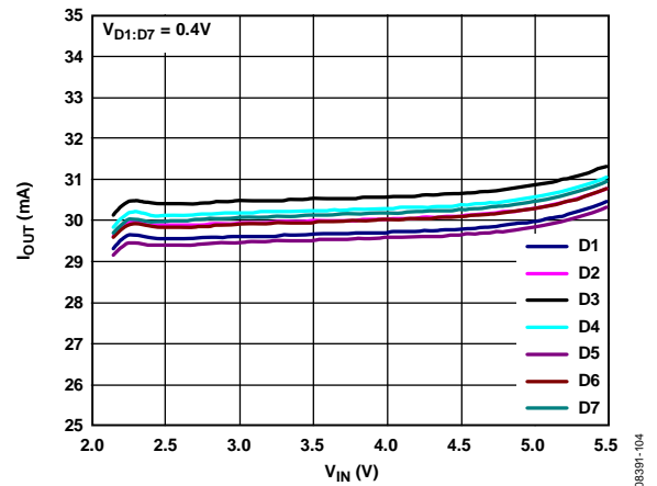
Figure 9. Typical Diode Current vs. V IN
