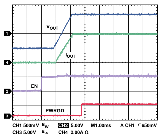
Figure 32. Channel 1/Channel 2 Soft Start with 4A Resistance Load, V_{IN} = 12V , V_{OUT} = 1.2V , f_{SW} = 600kHz , L = 1\mu H , C_{OUT} = 47\mu F \times 2
