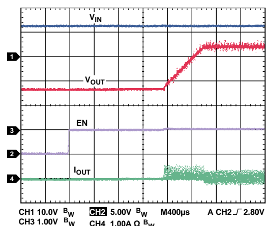
Figure 33. Startup with Precharged Output, V_{IN} = 12V , V_{OUT} = 3.3V
