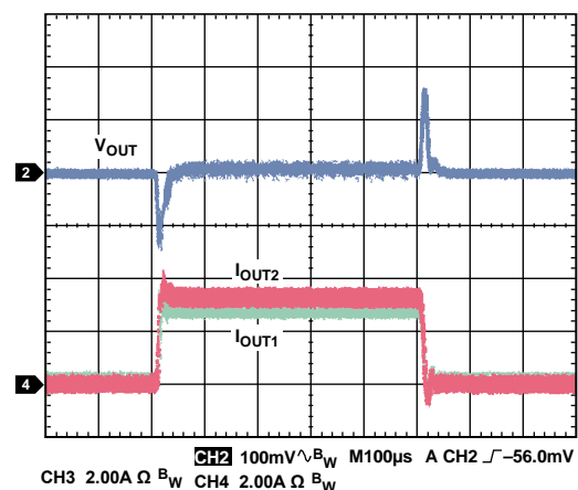
Figure 31. Load Transient, Channel 1/Channel 2 Parallel Output, 0A to 6A, V_{IN} = 12V , V_{OUT} = 3.3V , f_{SW} = 600kHz , L = 4.7\mu H , C_{OUT} = 47\mu F \times 4
