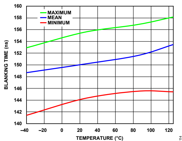
Figure 16. Blanking Time vs. Temperature
