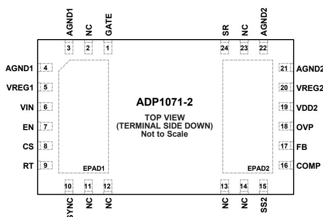
Figure 5. ADP1071-2 LGA Pin Configuration
