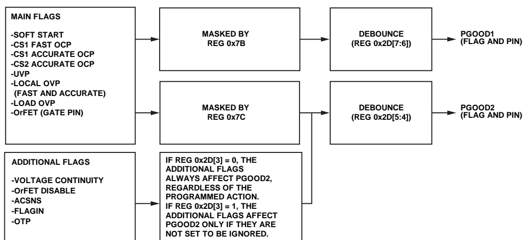
Figure 30. PGOOD1, PGOOD2 Programming
