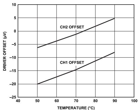
Figure 23. Driver Offset vs. Temperature
