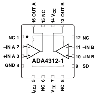
Figure 1. Thermally Enhanced, 4 mm × 4 mm, 16-Lead LFCSP
