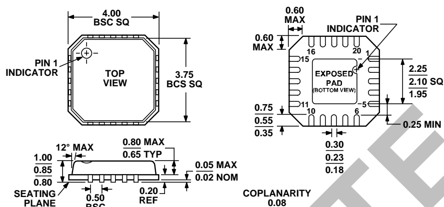
Figure 18. 20-Lead Lead Frame Chip Scale Package [LFCSP_VQ] 4 mm × 4 mm Body, Very Thin Quad (CP-20-1) Dimensions shown in millimeters
