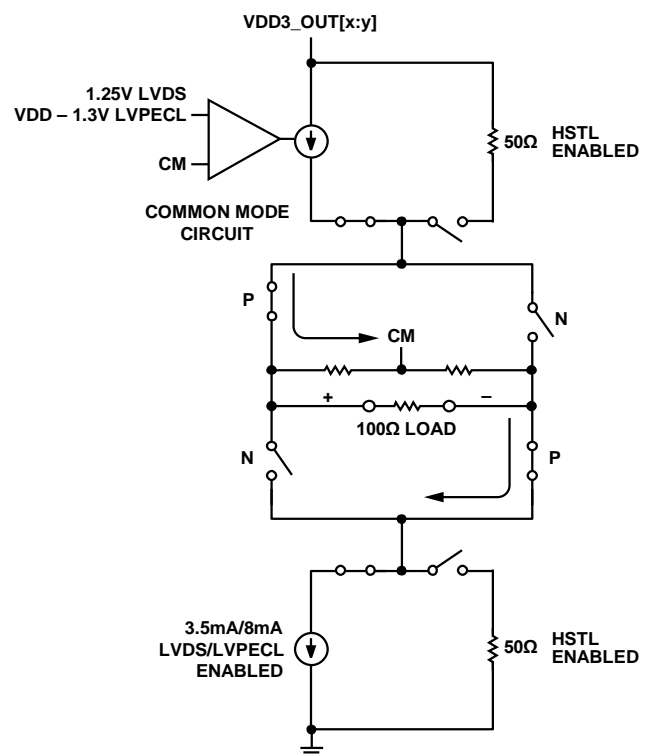
Figure 28. Multimode Driver
