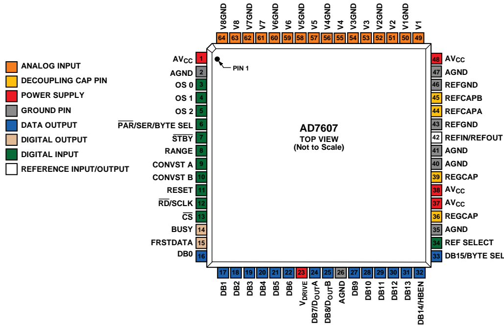
Figure 8. Pin Configuration
