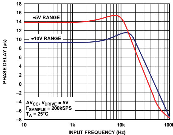
Figure 38. Analog Antialias Filter Phase Response
