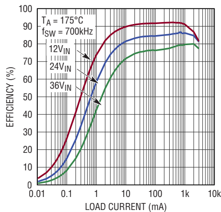
Efficiency at 175°C, V_{OUT} = 5V
