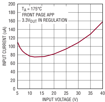
No Load Input Current at 175°C
