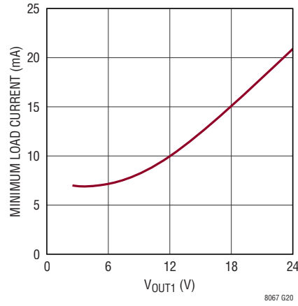
Minimum Load Current vs V_{OUT} Over Full Output Voltage Range
