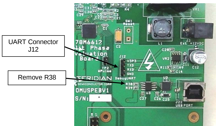
Figure 5: UART Connector
