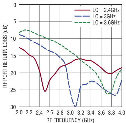
Figure 5. RF Port Return Loss
