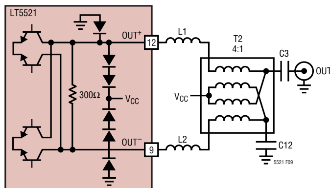
Figure 9. Simplified Output Circuit with External Matching Components
