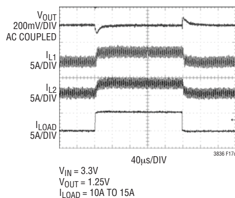
Figure 16c. Load Step
