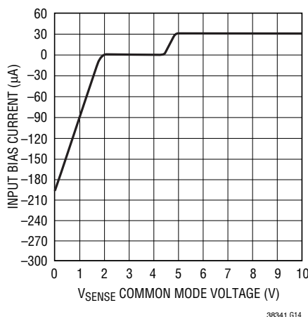
Figure 2. SENSE Pins Input Bias Current vs Common Mode (Output) Voltage
