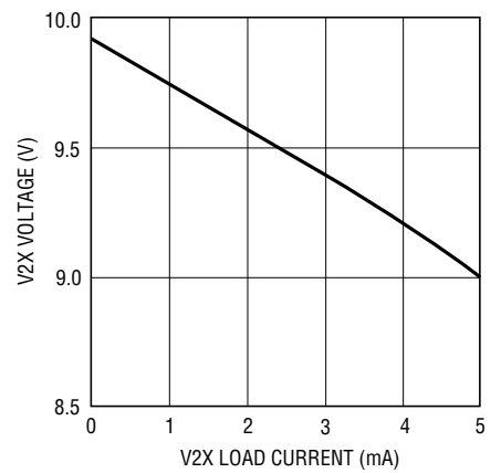
V2X Output Voltage vs V2X Load Current
