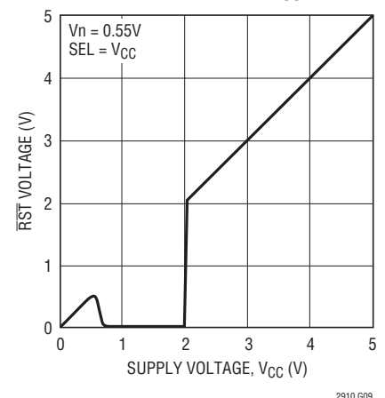
RST Output Voltage vs V_{CC}
