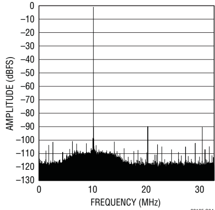
LTC2215 64k Point FFT, f_{IN} = 140.5\text{MHz} , -1dBFS
