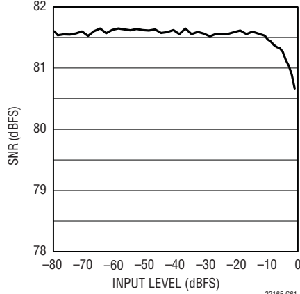
LTC2215 SNR vs Input Level, f_{IN} = 70.5\text{MHz}
