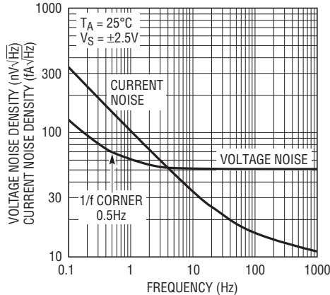
Noise Spectrum
