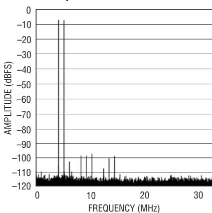
LTC2162: 64k Point 2-Tone FFT, f_{IN} = 69\text{MHz} , 70\text{MHz} , -7\text{dBFS} , 65Msps
