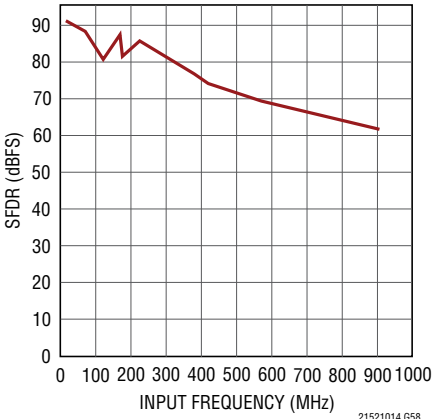
LTC2150-14: SFDR vs Input Frequency, -1dBFS, 1.5V Range, 170Msps
