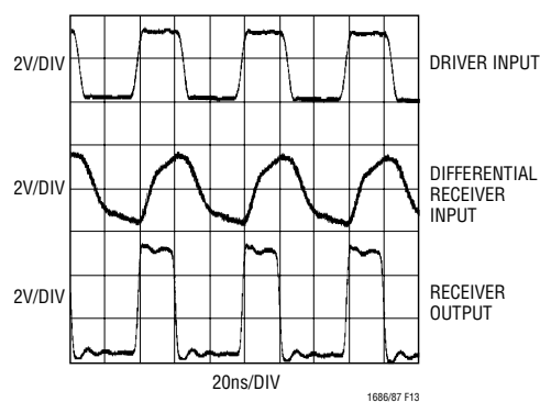
Figure 13. 100 Feet of Telephone Grade UTP: 30Mbps
