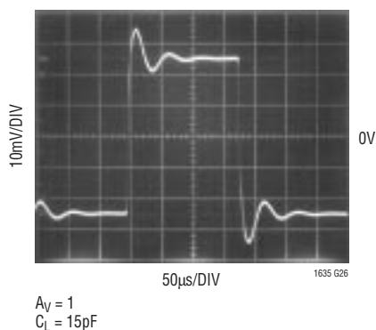
Small-Signal Transient Response V S = ±5V
