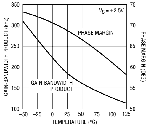
Gain-Bandwidth Product and Phase Margin vs Temperature
