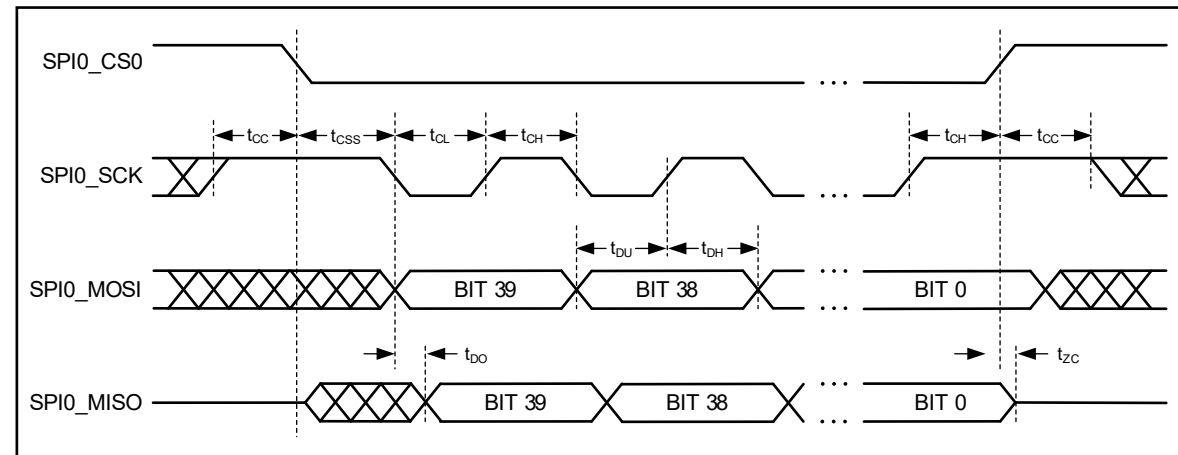
Figure 14. SPI Peripheral Timing Diagram in Bootloader Mode
