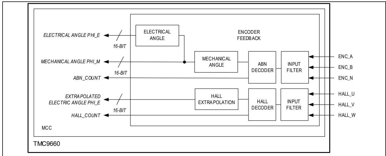
Figure 18. Encoder Feedback Engine
