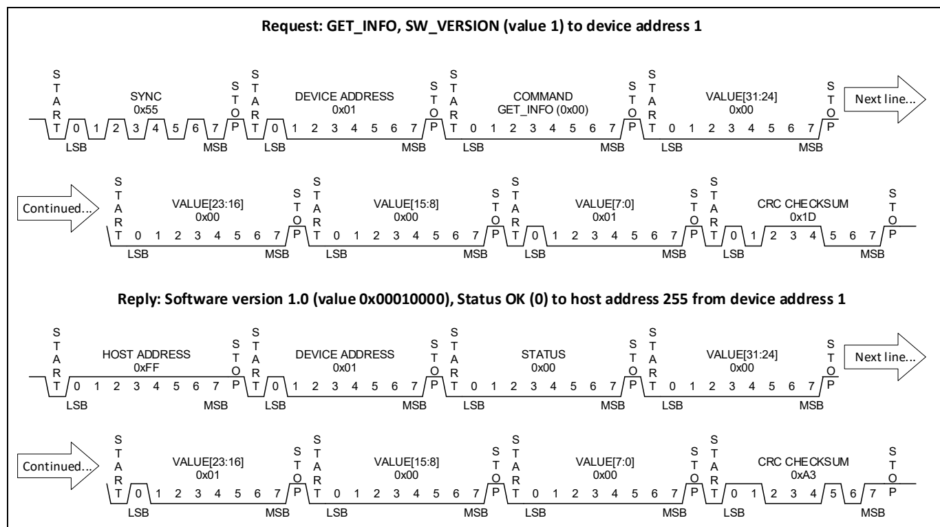
Figure 36. UART Example Request and Reply Pair
