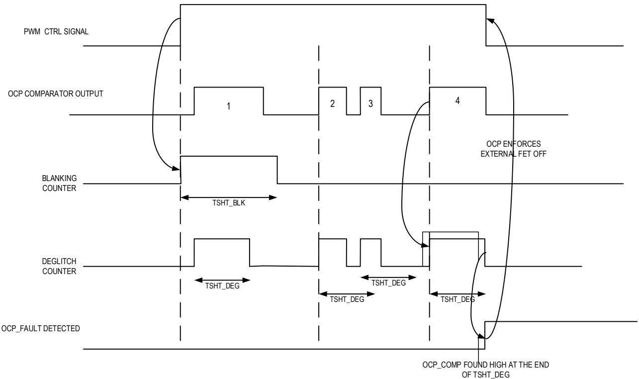
Figure 27. Blanking and Deglitch
