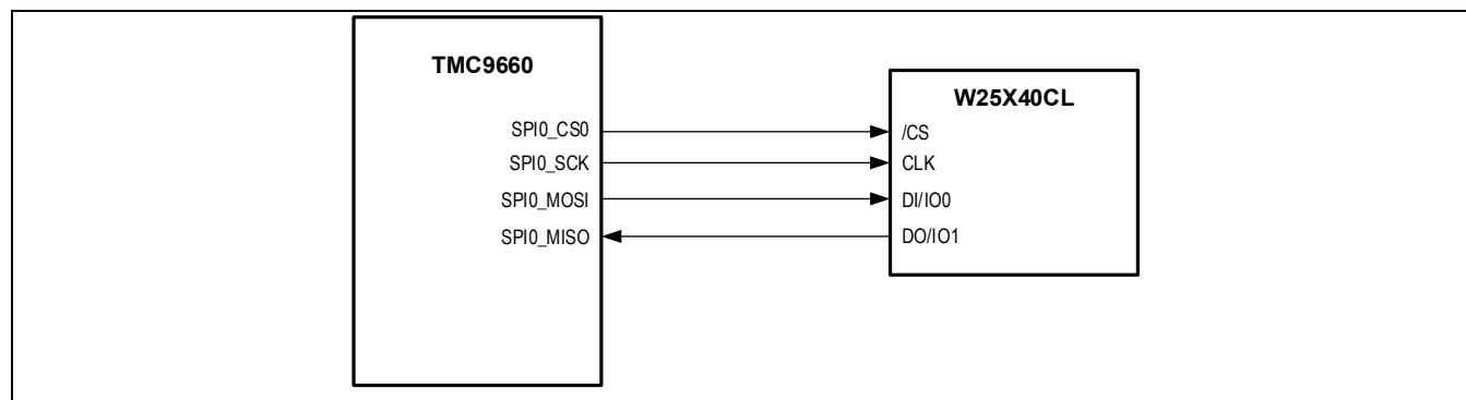
Figure 12. External Flash Memory Connected through SPI
