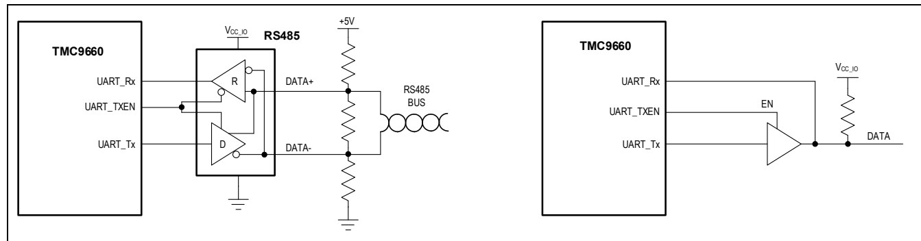
Figure 8. UART with External Transceiver
