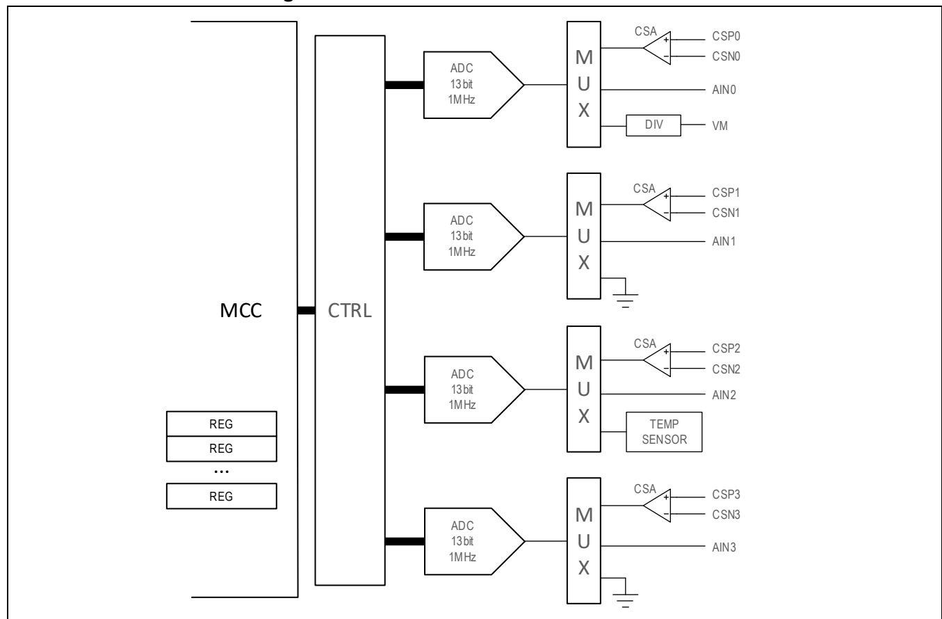
Figure 24. Measurement Unit Block Diagram
