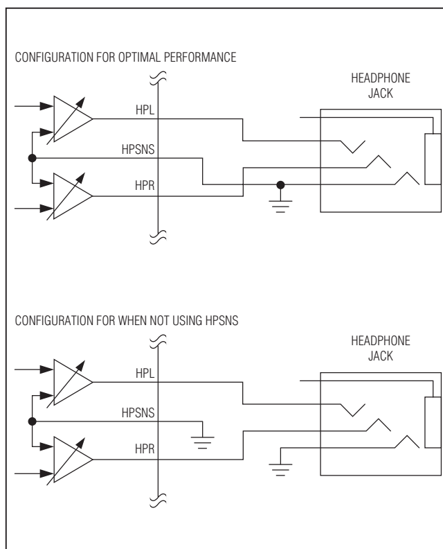
Figure 30. HPSNS Configurations
