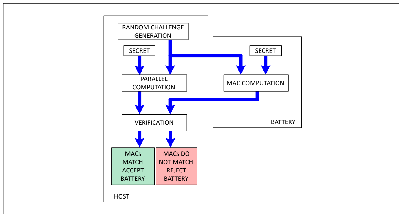
Figure 30. Procedure to Verify a Battery
