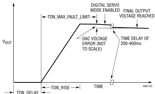
Figure 25. Timing Controlled V_{\text{OUT}} Rise
