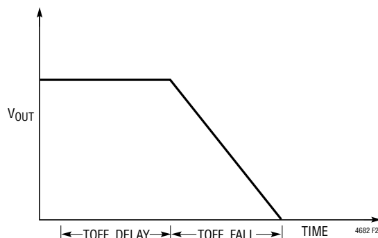
Figure 26. \text{TOFF\_DELAY} and \text{TOFF\_FALL}
