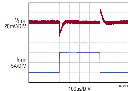
FIGURE 48 CIRCUIT C_{\text{OUT}} = 470\mu\text{F} \times 3 POSCAP, 100\mu\text{F} \times 4 CERAMIC R_{\text{COMP}} = 15\text{k} , E\text{A-}g_m = 3.02\text{mS} \text{COMPna} = 2.2\text{nF} , \text{COMPnb} = 150\text{pF} I_{\text{LIM}} RANGE HIGH, V_{\text{OUT}} RANGE LOW
