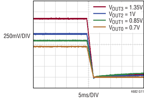
FIGURE 48 CIRCUIT, 12\text{V}_{\text{IN}} , 30\text{A} ON V_{\text{OUT0}} NO LOAD ON OTHER OUTPUTS AND 400\text{mV} PREBIAS ON V_{\text{OUT1}}
