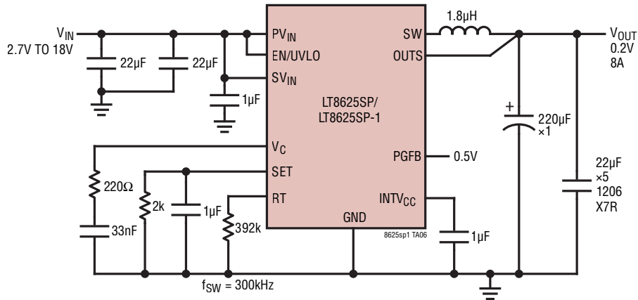
0.2V 8A 300kHz Step-Down Converter with Soft-Start
