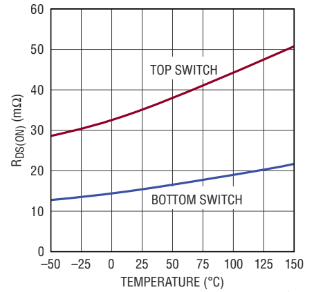
Switch R_{DS(ON)} vs Temperature
