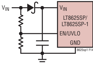
Figure 14. Reverse V_{\text{IN}} Protection
