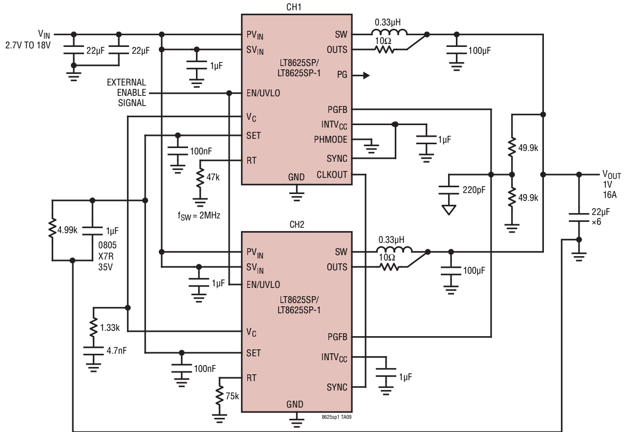
1V 16A 2MHz 2-Phase Step-Down Converter With Soft-Start, Fast Start-Up, and Power Good
