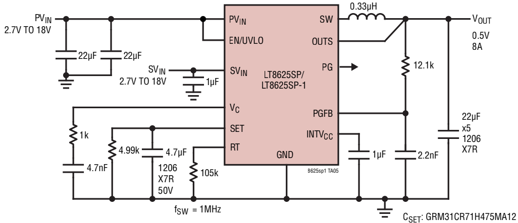
0.5V 8A 1MHz Step-Down Converter with Soft-Start, Fast Start-Up and Power Good
