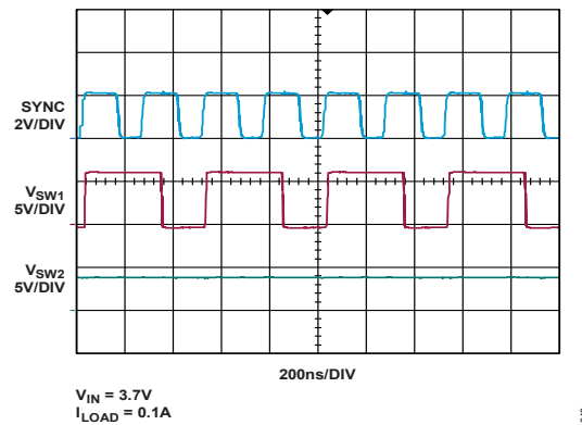
Figure 11. Switching Waveforms, Light Load 1-Phase Operation with SYNC
