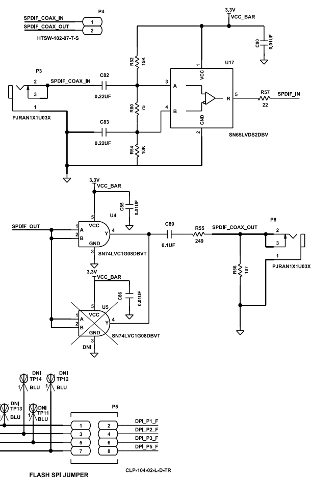
Figure 5. EVAL-ADSP1802EBZ Schematics, Page 3
