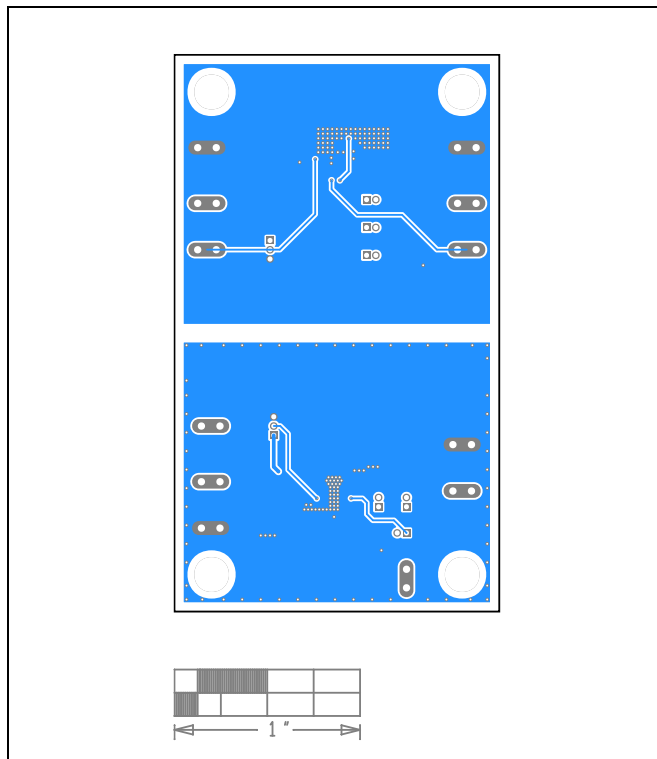
ADPL44001EVKIT—Layer 2
