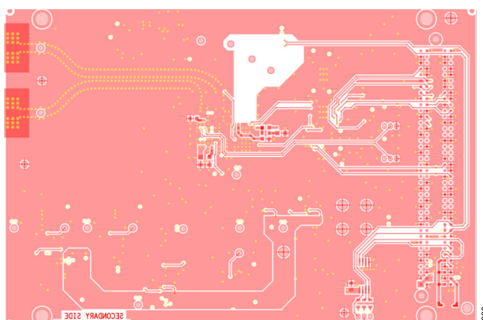
Figure 26. EVAL-ADAQ4224-FMCZ, Bottom Layer 4
