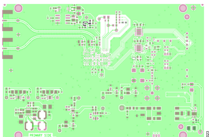
Figure 23. EVAL-ADAQ4224-FMCZ, Top Layer 1
