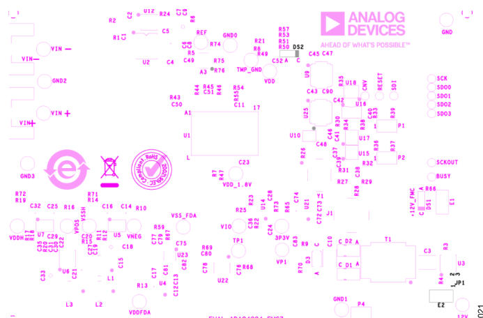
Figure 21. EVAL-ADAQ4224-FMCZ Silkscreen, Top Layer
