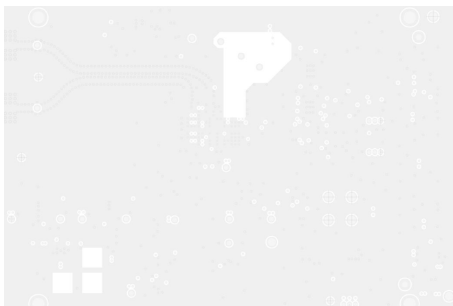
Figure 24. EVAL-ADAQ4224-FMCZ, Ground Layer 2
