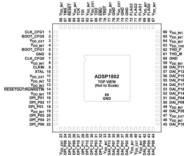
Figure 30. Pin Configuration
