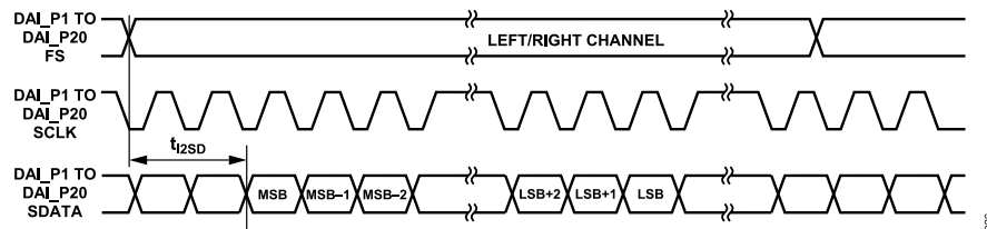
Figure 23. I 2 S-Justified Mode
