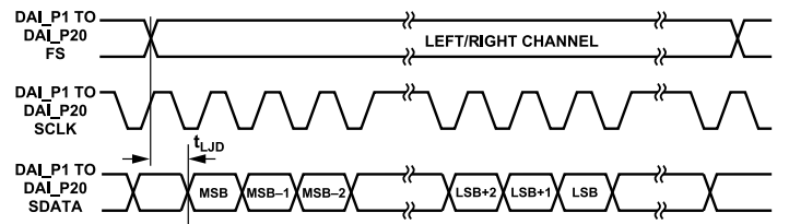
Figure 24. Left-Justified Mode
