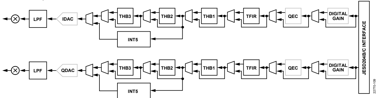
Figure 110. Transmit Signal Path Diagram
