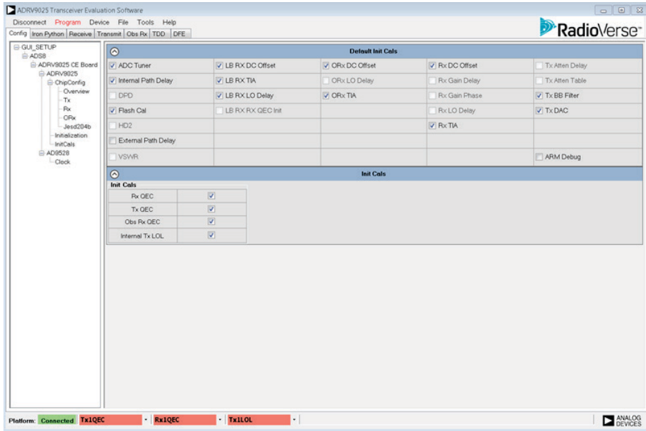
Figure 174. InitCals Tab with Default Settings
