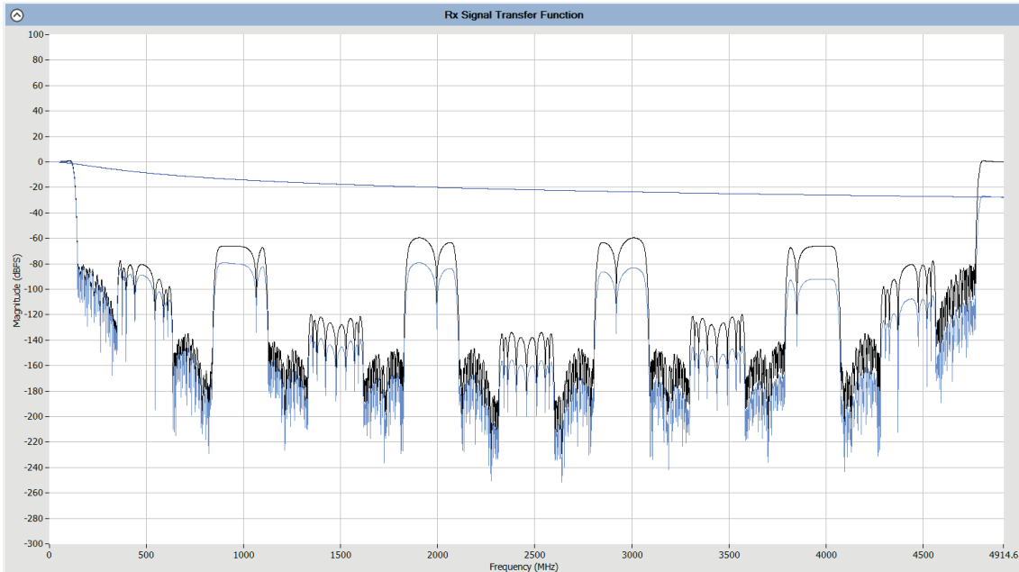
Figure 109. Receive Signal Transfer Function
