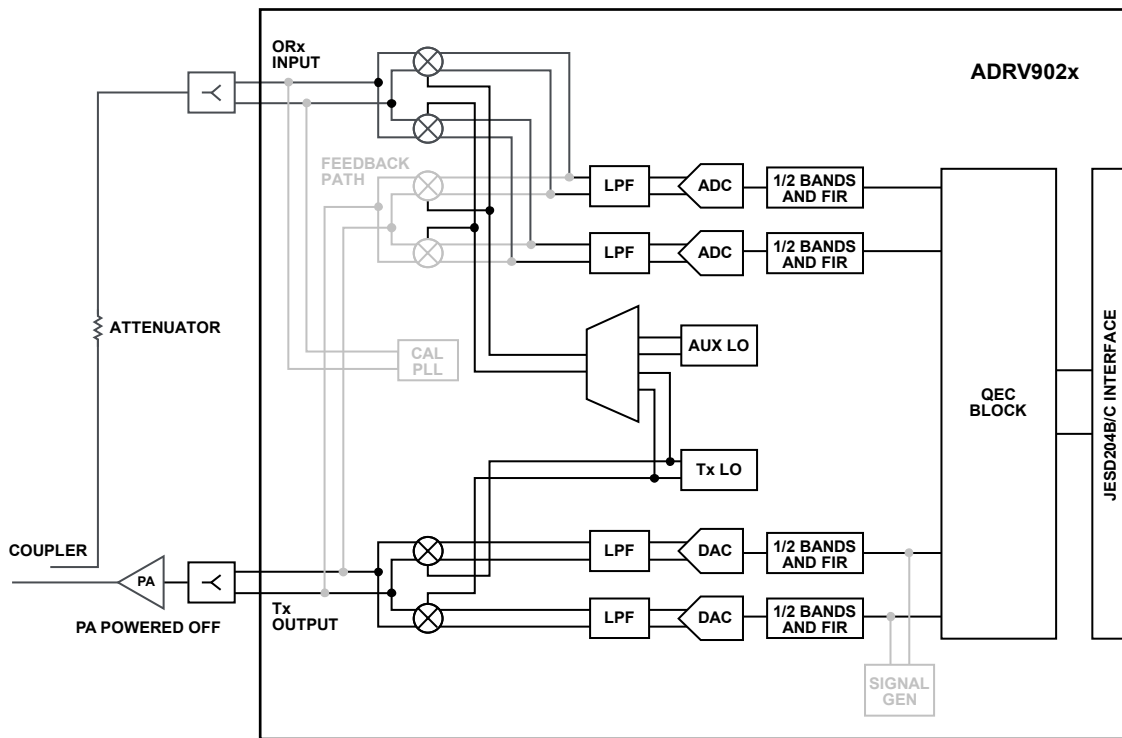
Figure 59. Transmitter LOL Tracking Configuration
