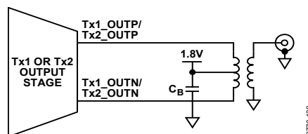
Figure 133. RF Transmitter Interface Configuration A
