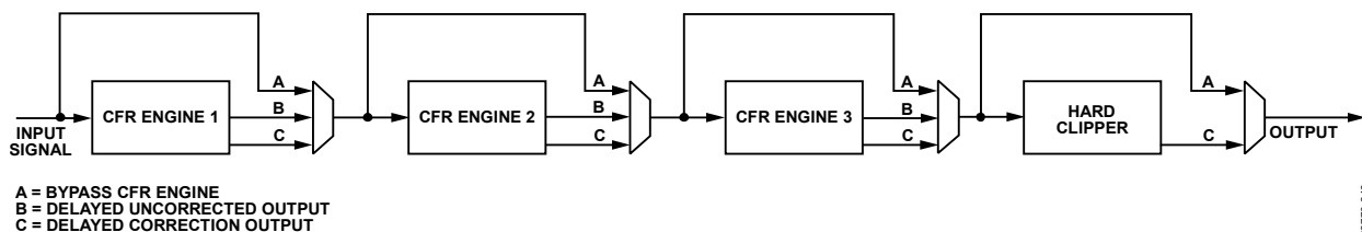
Figure 254. ADRV9029 Cascaded CFR Engine Blocks
