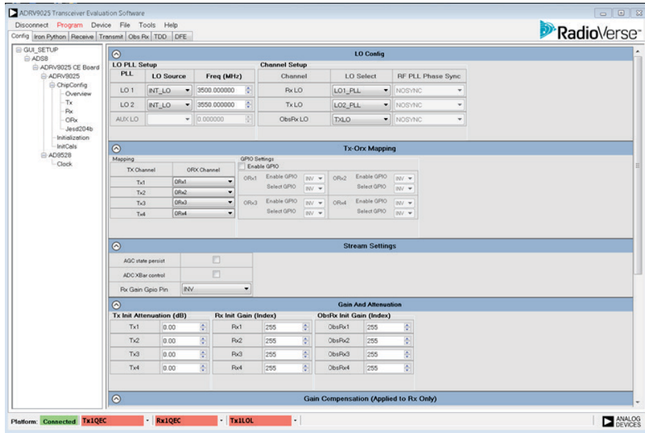
Figure 173. Initialization Configuration Tab
