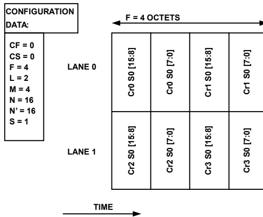
Figure 20. JESD204B Deframer Configuration (M = 4, L = 2)
