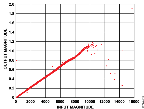
Figure 227. Effect of Optimum DPD Regularization on DPD Stability
