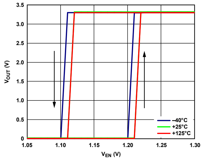
Figure 28. Typical V_{OUT} Response to EN Pin Operation
