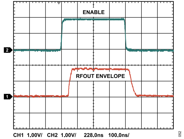
Figure 52. On and Off Response of the ADL8140 RF Output Envelope When the IN Pin of the ADG719 Is Pulsed, P_{OUT} = 5 dBm at 12 GHz
