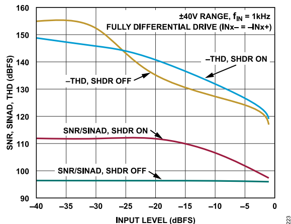
Figure 23. SNR, SINAD, and THD vs. Input Level
