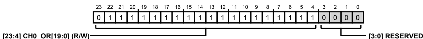
Figure 104. Address: 0x32 to Address 0x34, Reset: 0x7FFF0, Name: CH0_OR
