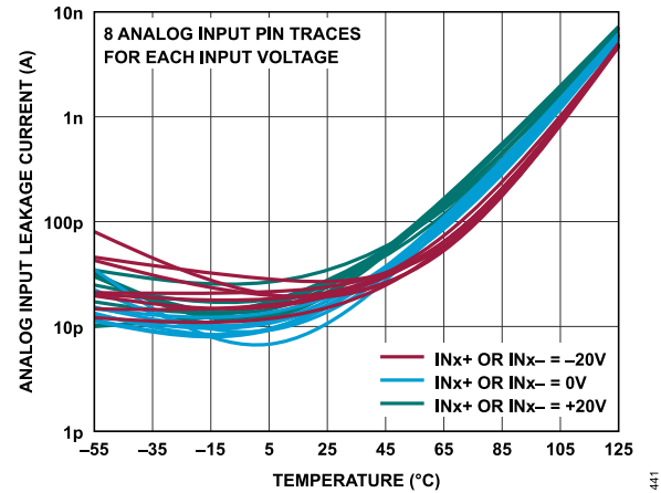
Figure 41. Analog Input Leakage Current vs. Temperature
