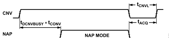
Figure 62. Nap Mode Timing for the AD4854
