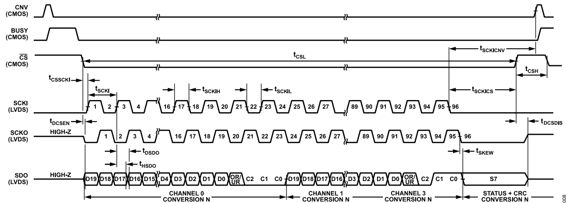
Figure 7. LVDS Conversion Data Bus Timing
