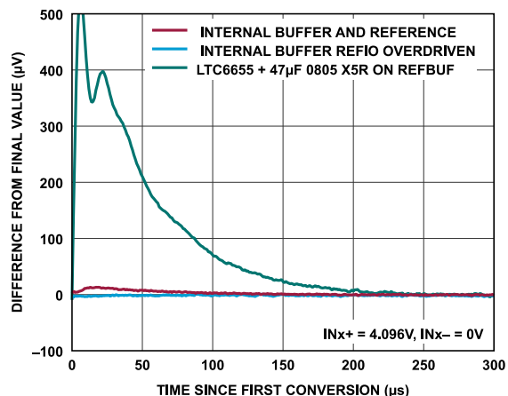
Figure 36. Burst Conversion Response, f_s = 1\text{MSPS}
