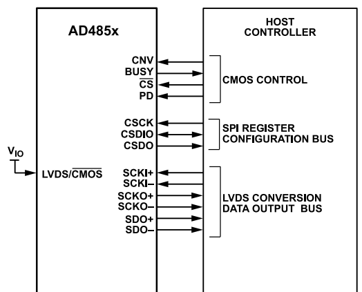
Figure 67. LVDS Conversion Data Output Mode for the AD4854
