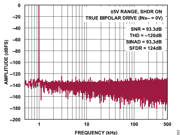
Figure 22. FFT, 1MSPS, f_{IN} = 1\text{kHz} , \pm 5\text{V} Range
