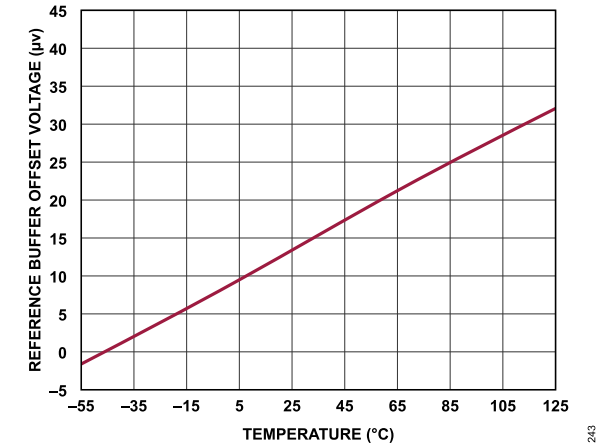
Figure 43. Reference Buffer Offset Voltage vs. Temperature
