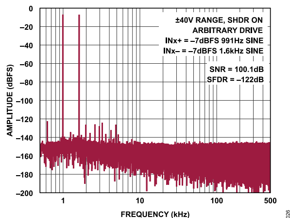
Figure 25. FFT, 1MSPS, f_{IN+} = 991\text{Hz} , f_{IN-} = 1.6\text{kHz} , \pm 40\text{V} Range
