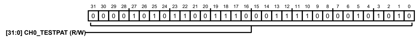
Figure 106. Address: 0x38 to Address:0x3B, Reset: 0x0ACE3C2A, Name: CH0_TESTPAT
