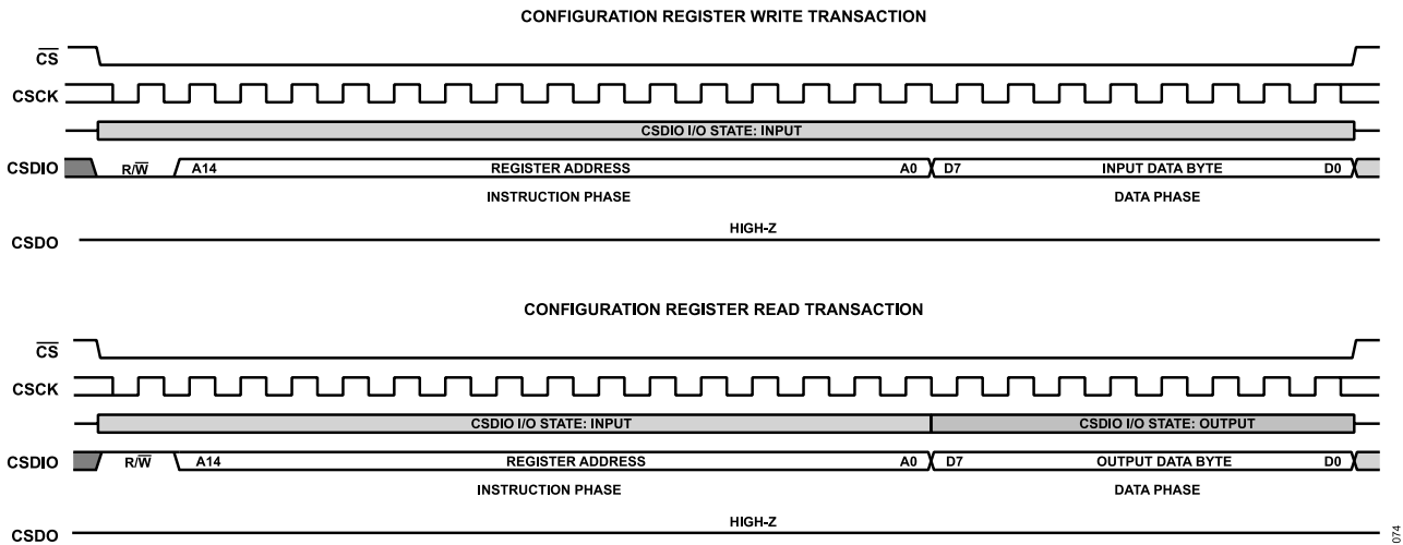
Figure 73. 3-Wire SPI Register Configuration Bus Frame
