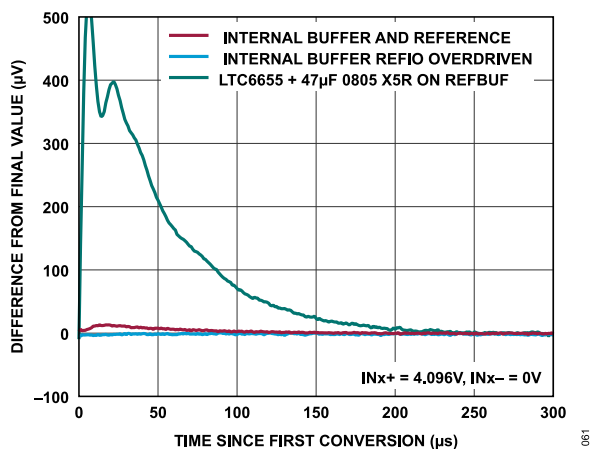
Figure 60. Burst Conversion Response of the AD4853, f_s = 1MSPS
