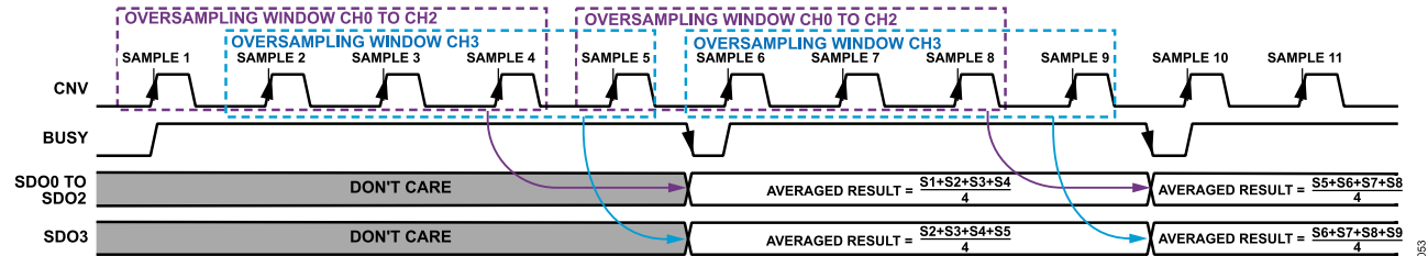
Figure 52. Oversampling Mode with 4× Oversampling Ratio (OS_RATIO = 0x1), Channel 3 Averages Phase-Shifted by One Sample (CH3_PHASE = 0x0001)
