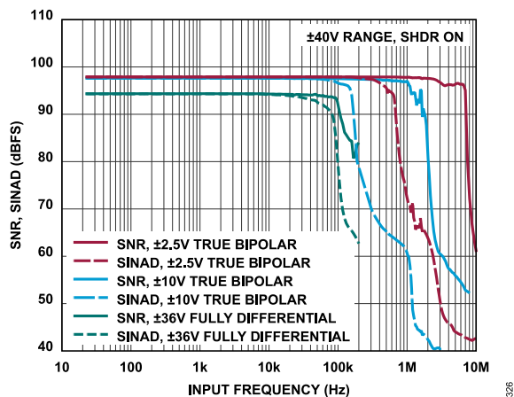
Figure 26. SNR and SINAD vs. Input Frequency
