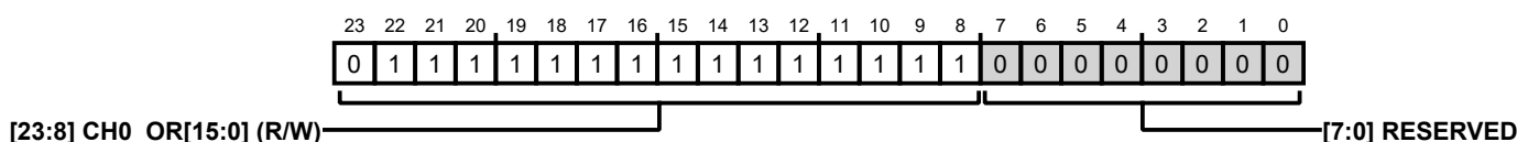
Figure 104. Address: 0x32 to Address 0x34, Reset: 0x7FFF00, Name: CH0_OR
