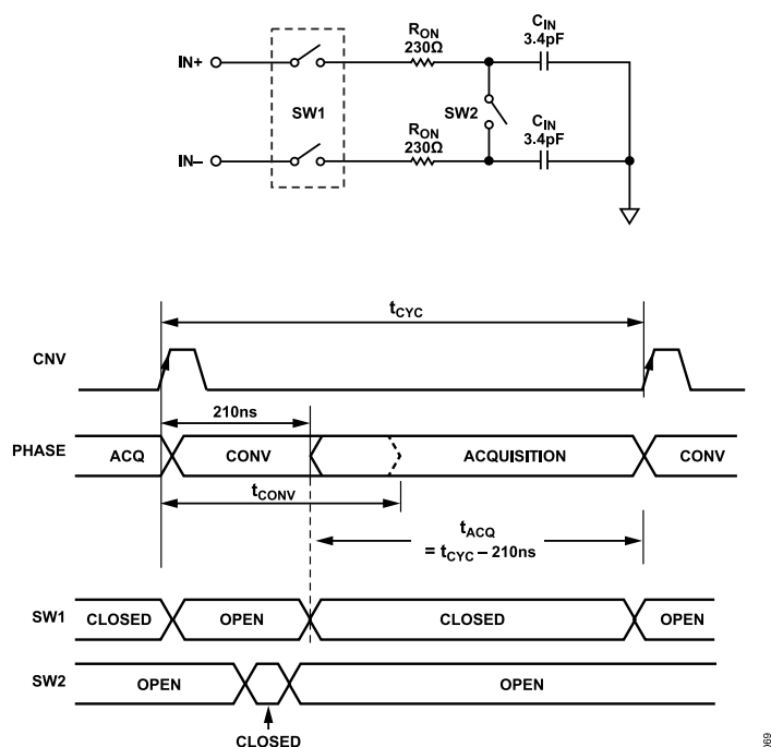
Figure 69. AD4052 Equivalent Input Load Model
