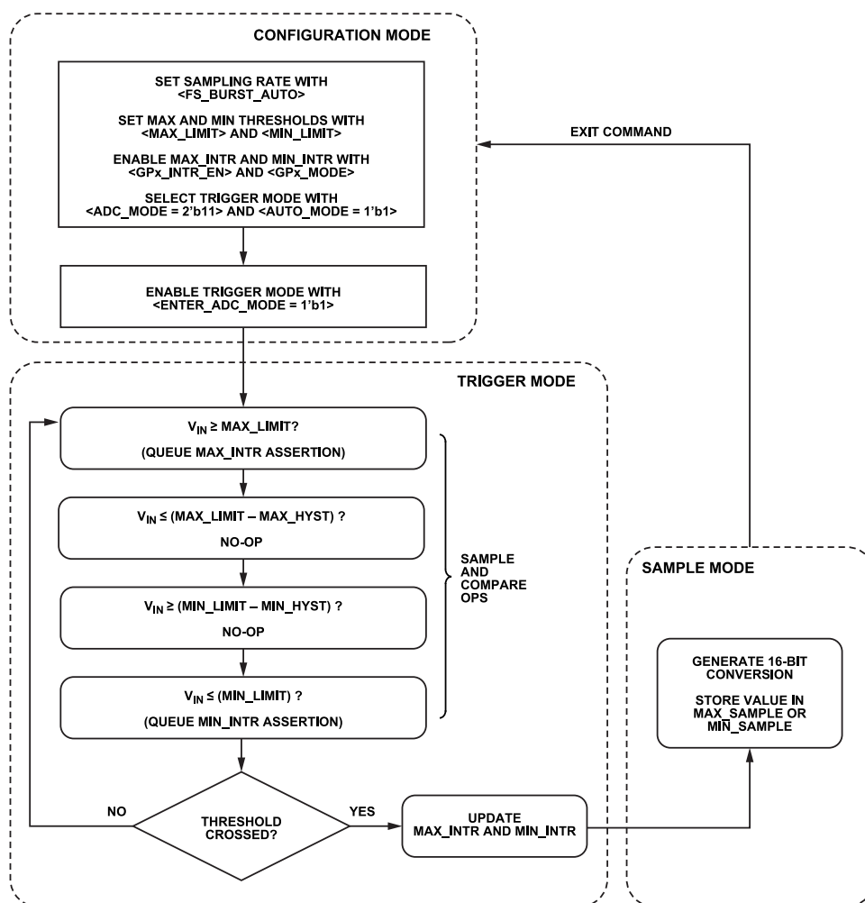
Figure 57. Trigger Mode Flowchart
